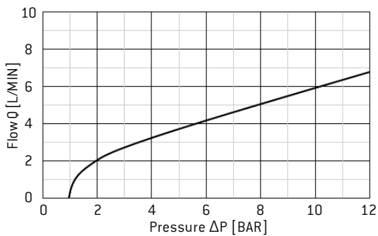
Valve Characteristics ( \Delta P vs. Flow), \varnothing 5.5 mm. RF, 1 bar cracking pressure (T = 50°C, Hydraulic Oil HLP46)
