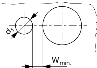
Wall Thickness Between Bores
