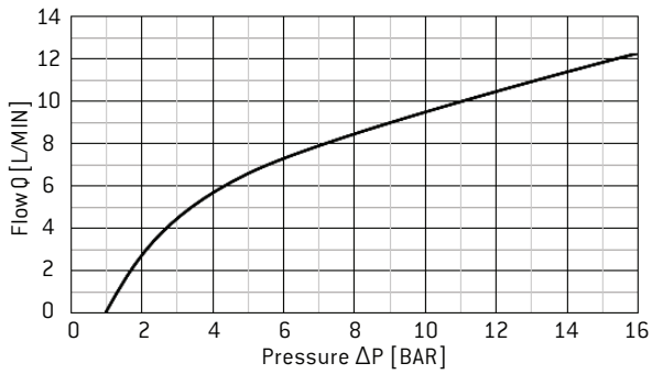
Valve Characteristics ( \Delta P vs. Flow), \varnothing 8.0 mm. FF, 1 bar cracking pressure (T = 50°C, Hydraulic Oil HLP46)
