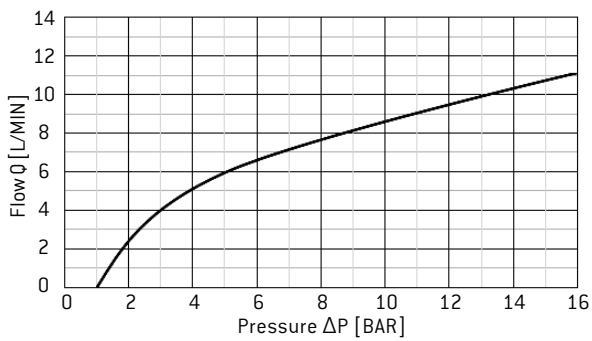
Valve Characteristics ( \Delta P vs. Flow), \varnothing 8.0 mm. RF, 1 bar cracking pressure (T = 50°C, Hydraulic Oil HLP46)
